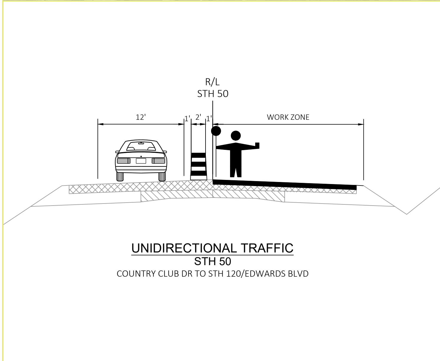
SEGMENT 4 (RESURFACE) WORK ZONE METHOD STAGING - TRAFFIC UNDER FLAGGING OPERATION
