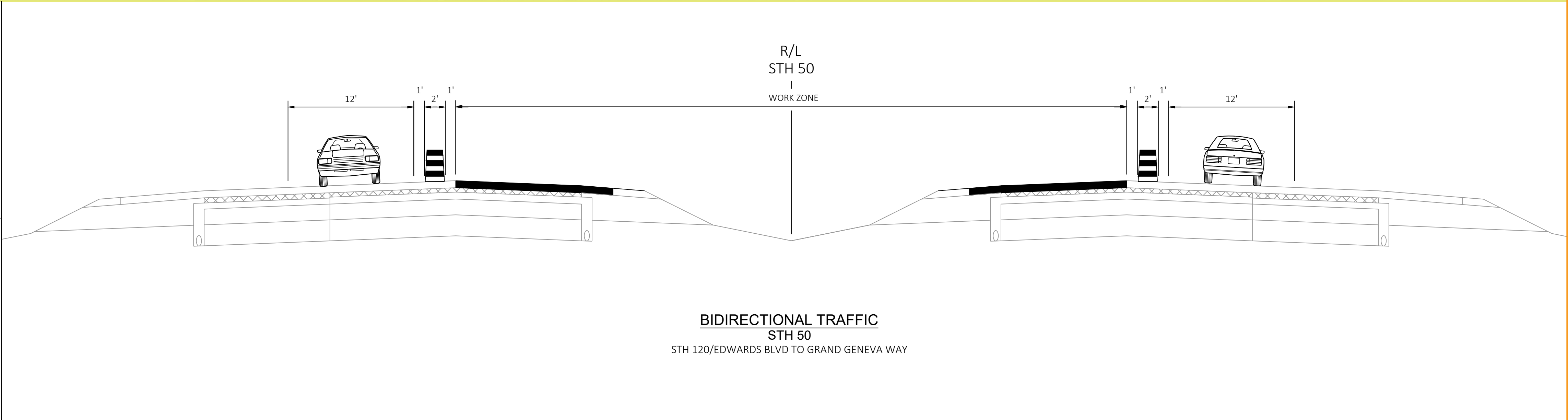
SEGMENT 5 (RESURFACE) WORK ZONE METHOD STAGING - BI-DIRECTIONAL TRAFFIC WITH LANE CLOSURES
